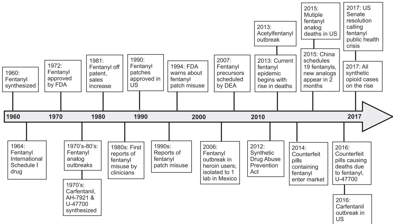
Fig. 2. Timeline of select synthetic opioid events.
